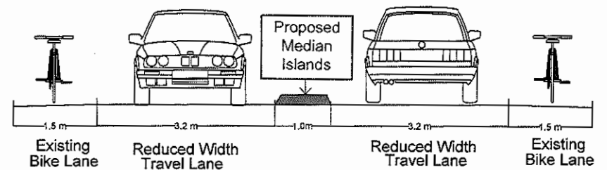
Cross-Section at Proposed Median Islands
