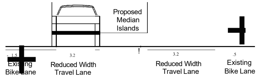
Cross-Section at Proposed Median Islands
