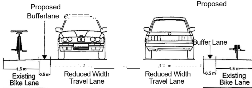
Typical Cross-Section without Median Islands
