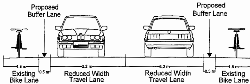
Typical Cross-Section without Median Islands
