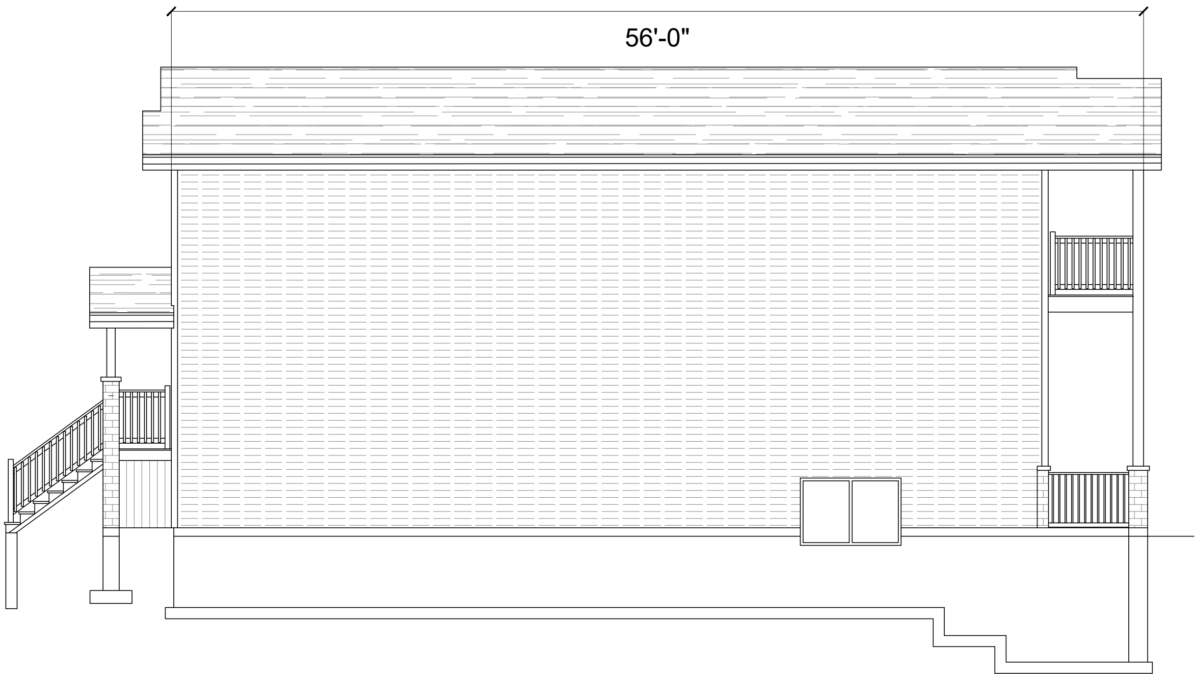
EXTERNAL ELEVATIONS (FACING NEIGHBOURS)
