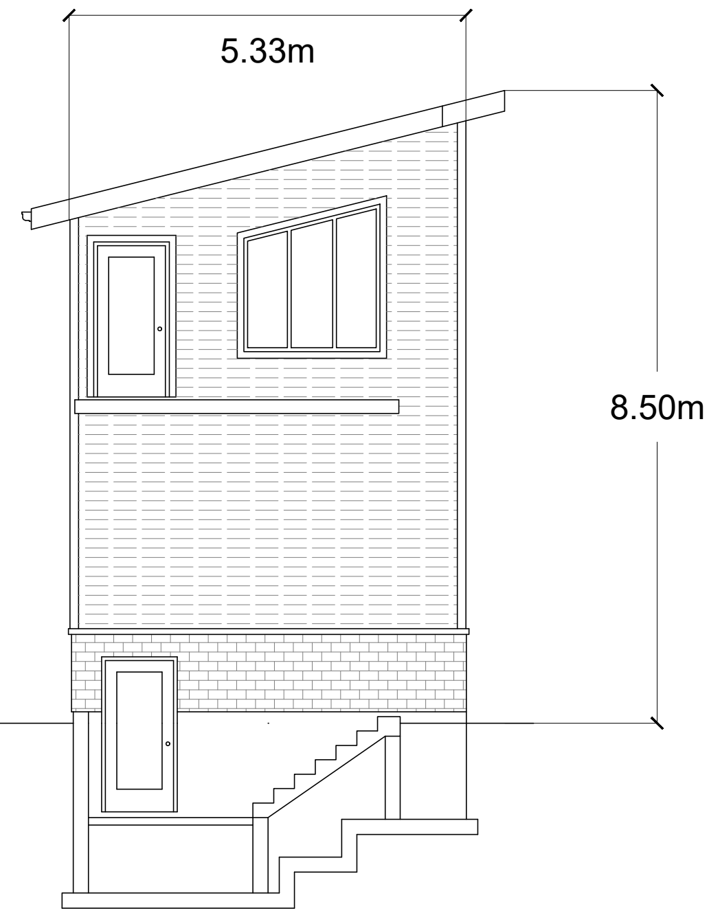
WEST ELEVATION
