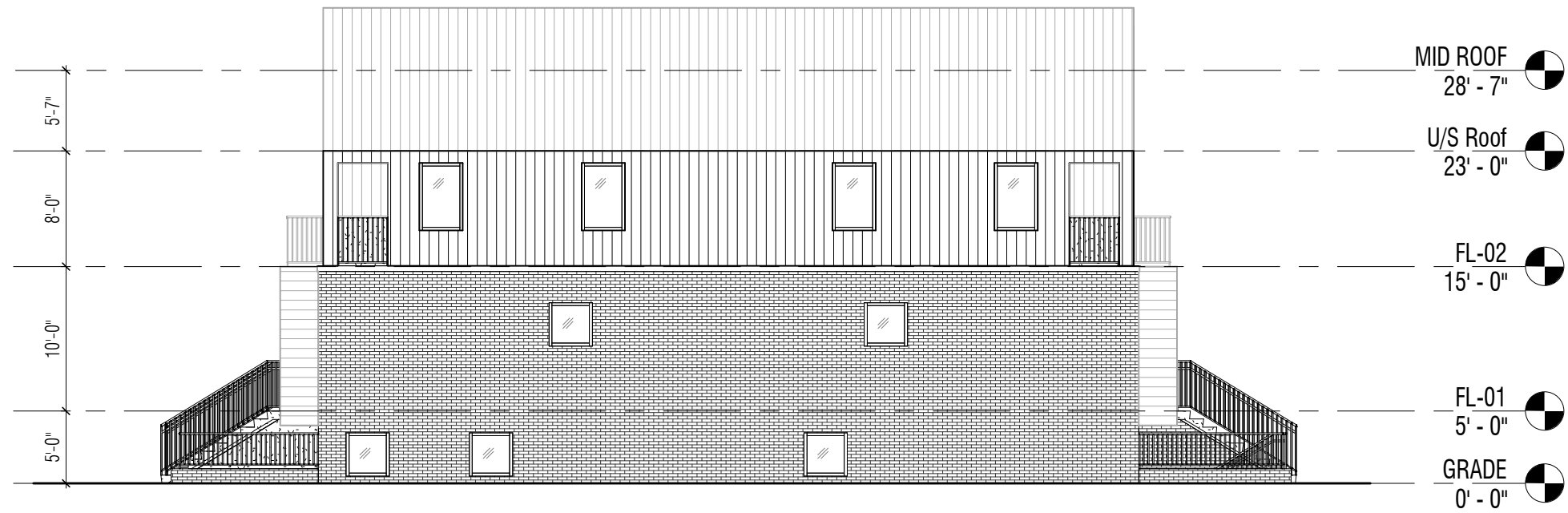
1 EAST ELEVATION SK6 3/32" = 1'-0"
