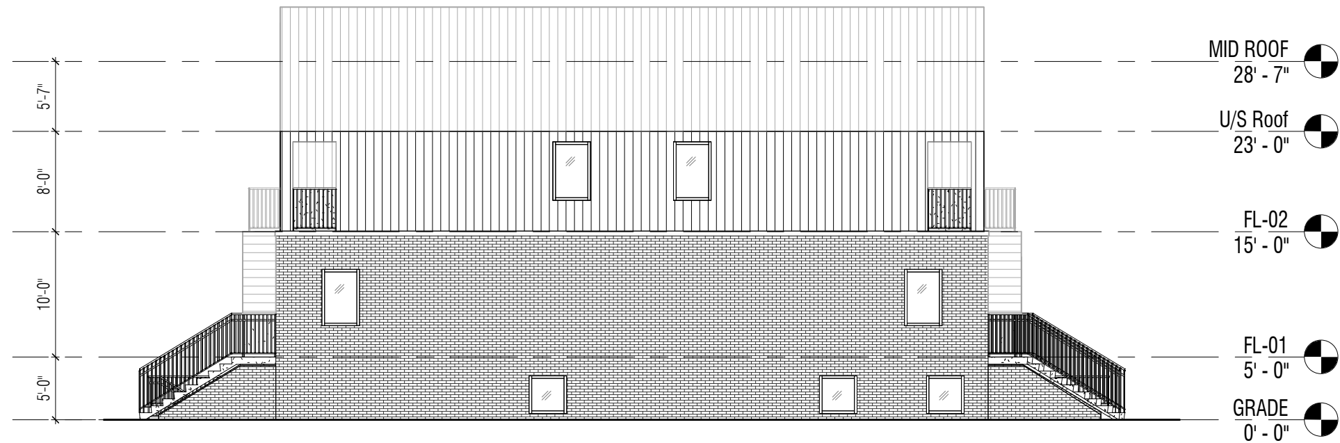
2 WEST ELEVATION SK6 3/32" = 1'-0"
