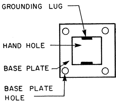
BASE DETAIL
