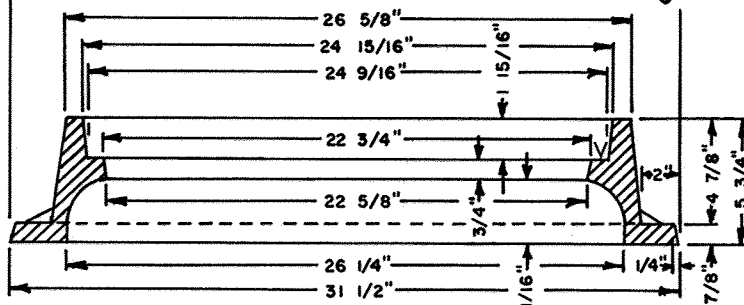
FRAME SECTION A-A
