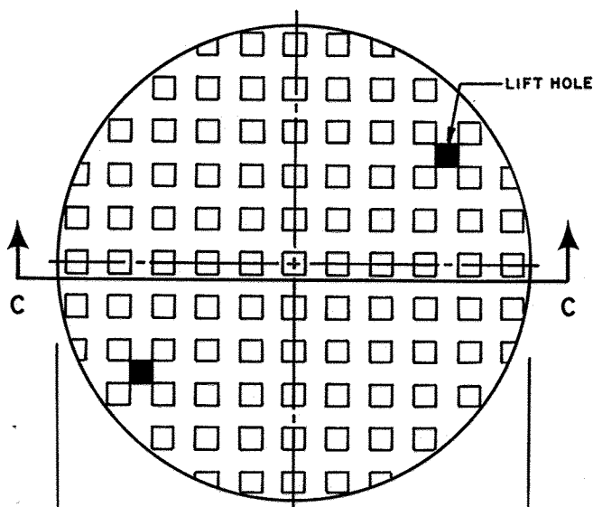
COVER PLAN
