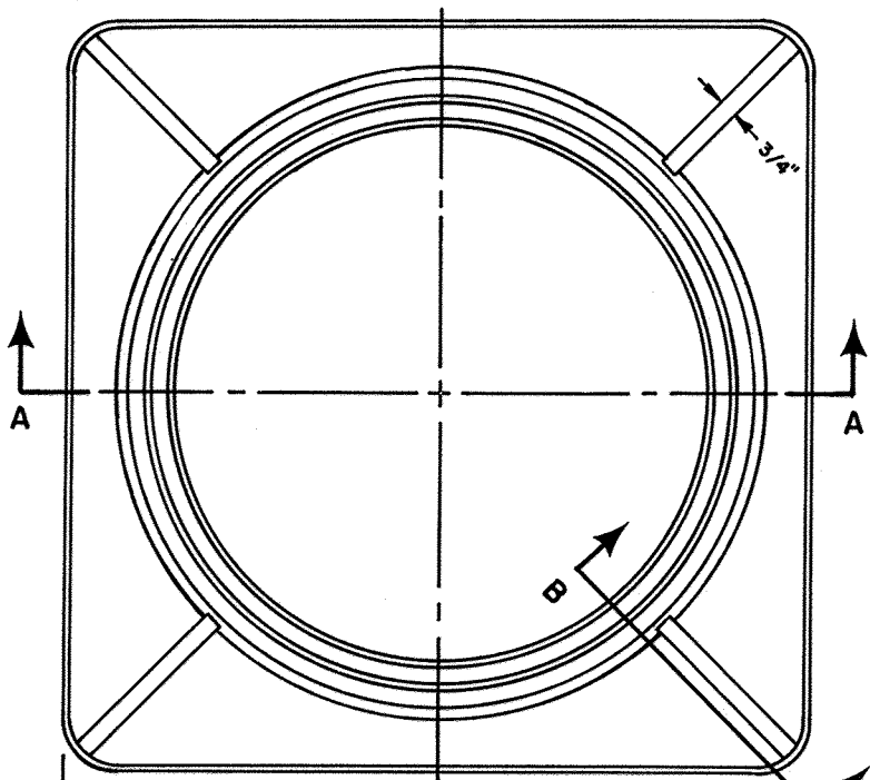
FRAME PLAN
