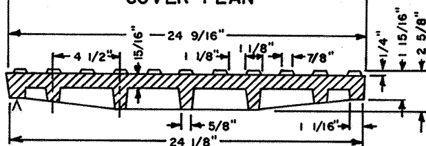
COVER SECTION C-C
