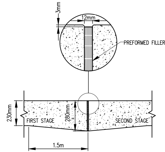
TYPE C TRANSVERSE CONSTRUCTION JOINT
