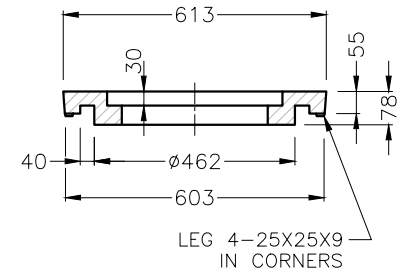
SECTION D-D ROUND COVER (NTS)
